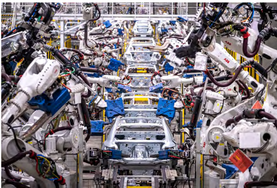
Assembly robots put together car bodies in the body shop at VinFast manufacturing plant in Haiphong.
